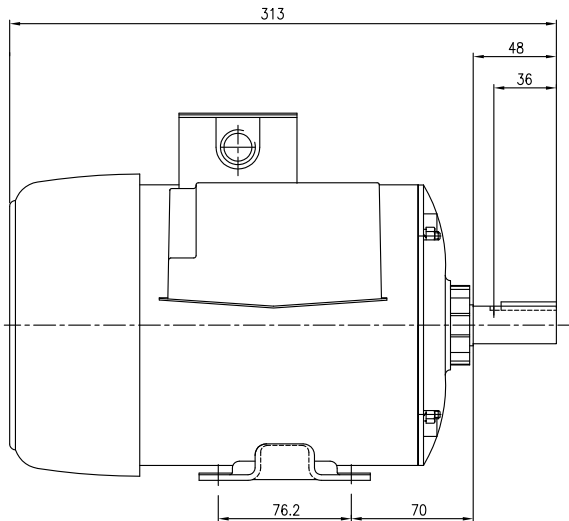
Enclosure - TEFC and DPFC
