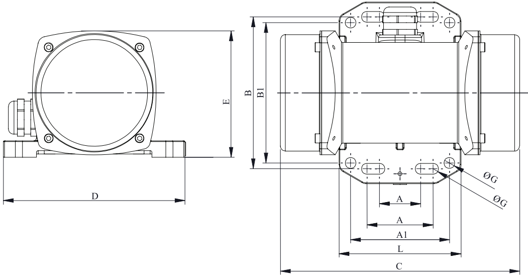
FIGURE F DIMENSION DRAWING
