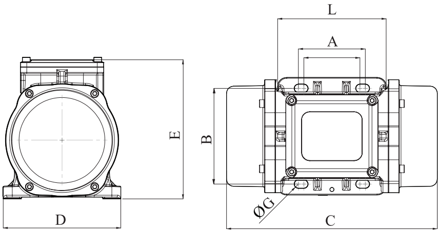
FIGURE B DIMENSION DRAWING
