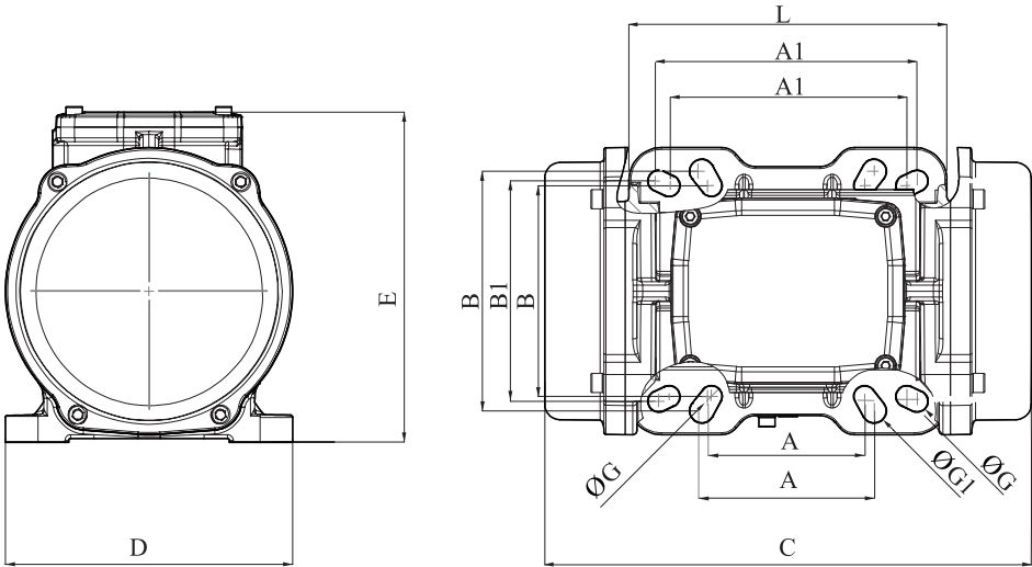
FIGURE C DIMENSION DRAWING
