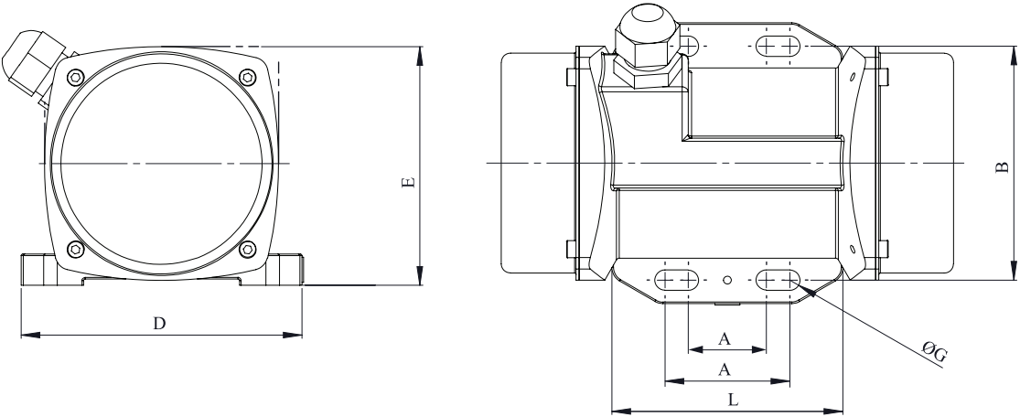
FIGURE I MICRO DIMENSIONS DRAWING
