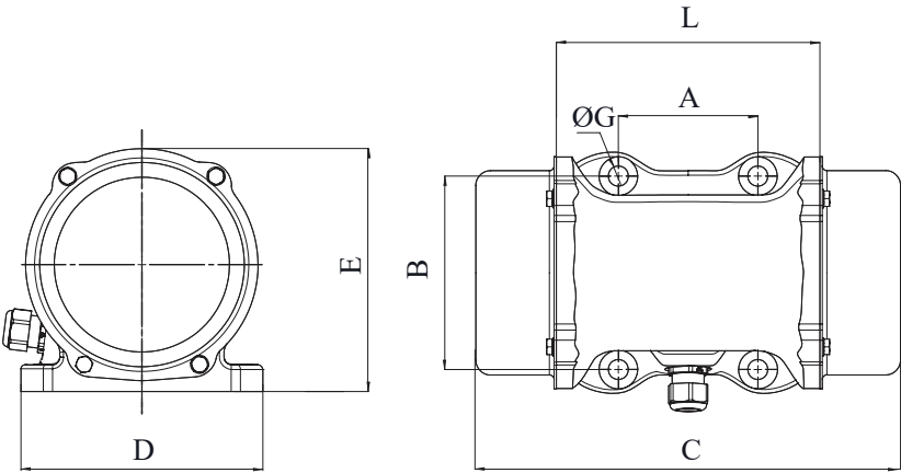
FIGURE P DIMENSION DRAWING
