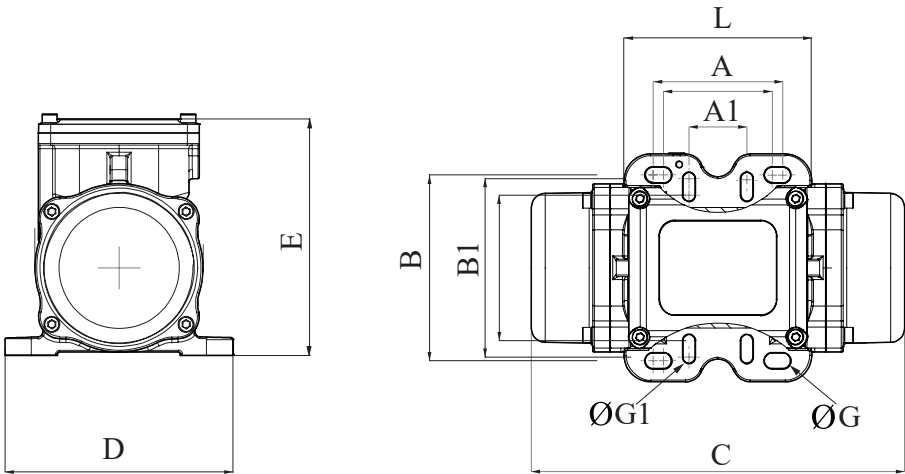
FIGURE A DIMENSION DRAWING
