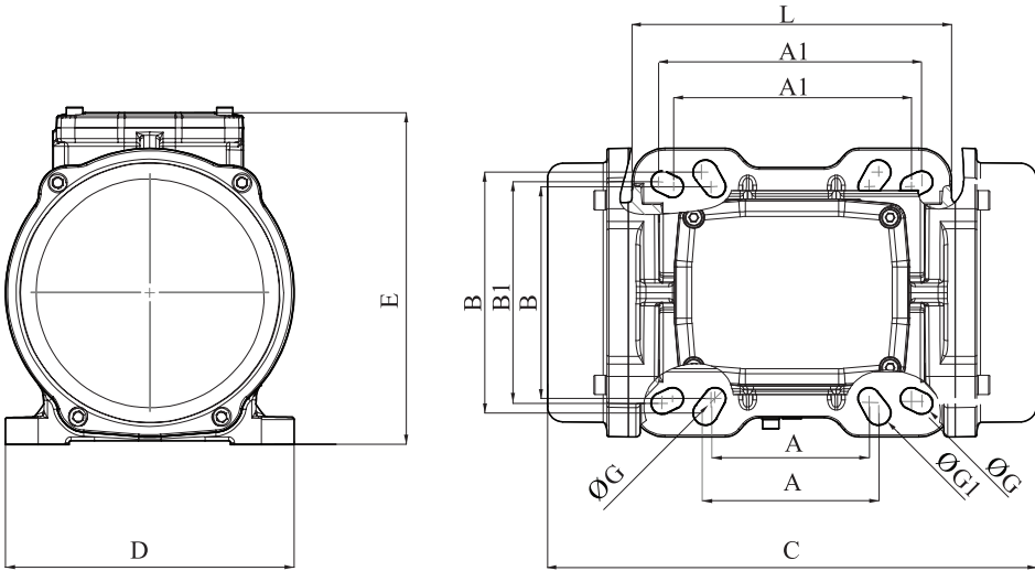
FIGURE C DIMENSION DRAWING
