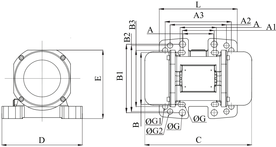
FIGURE G DIMENSION DRAWING
