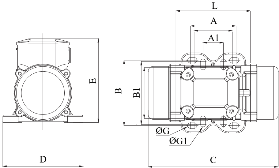
FIGURE A DIMENSION DRAWING
