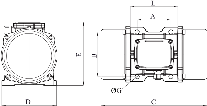
FIGURE D1 DIMENSION DRAWING
